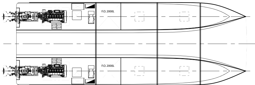
BOTTOM PLAN
