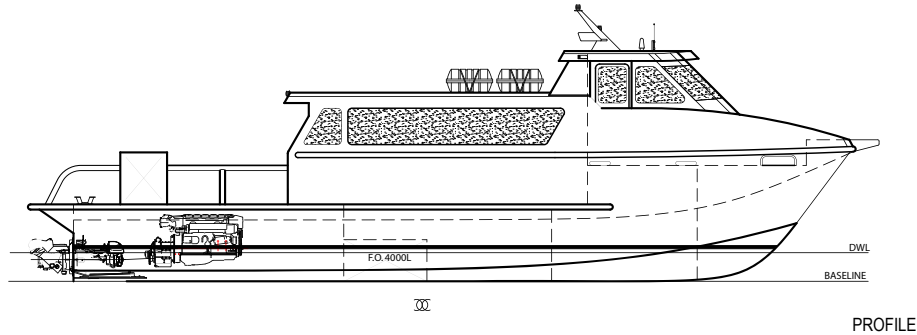
PROFILE
