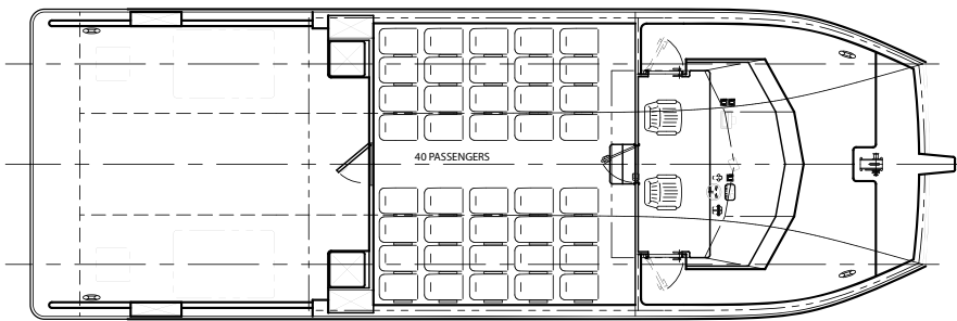
PLAN ON MAIN DECK
